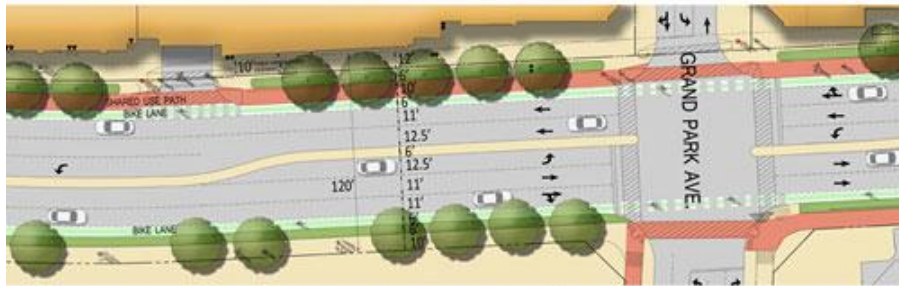
MASTER PLAN STREET SECTION
